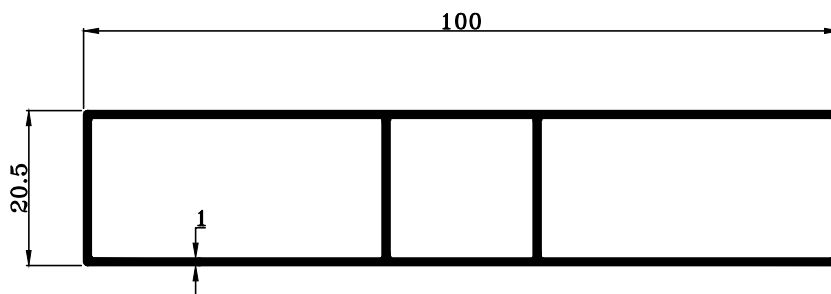
TRT-1435 W : 0.739 KG./M.
